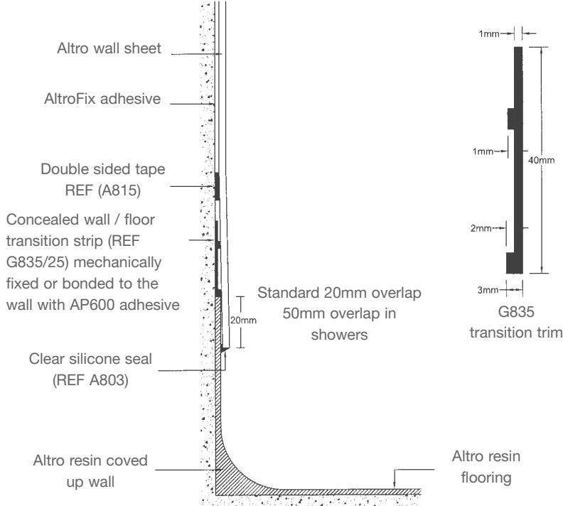
Concealed transition strip
